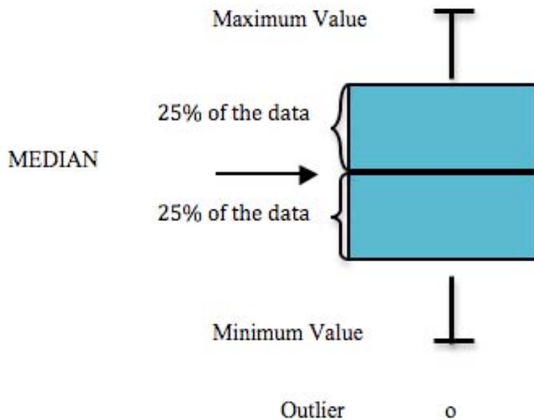
Figure 25: Diagram of the components of a box plot
